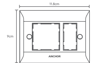
Single Mounting Plate Design
